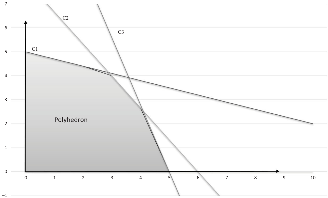
Fig. 2. Linear programming as a graph in a simplified model.
